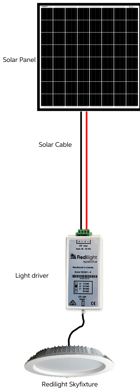
Single Skyfixture
