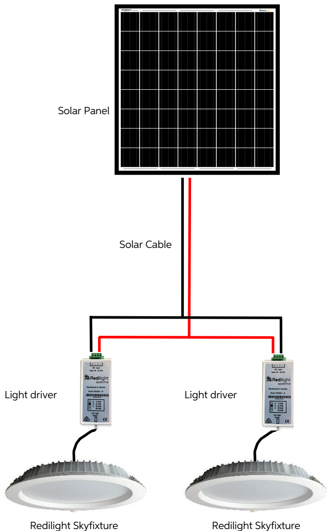
Double Skyfixture
