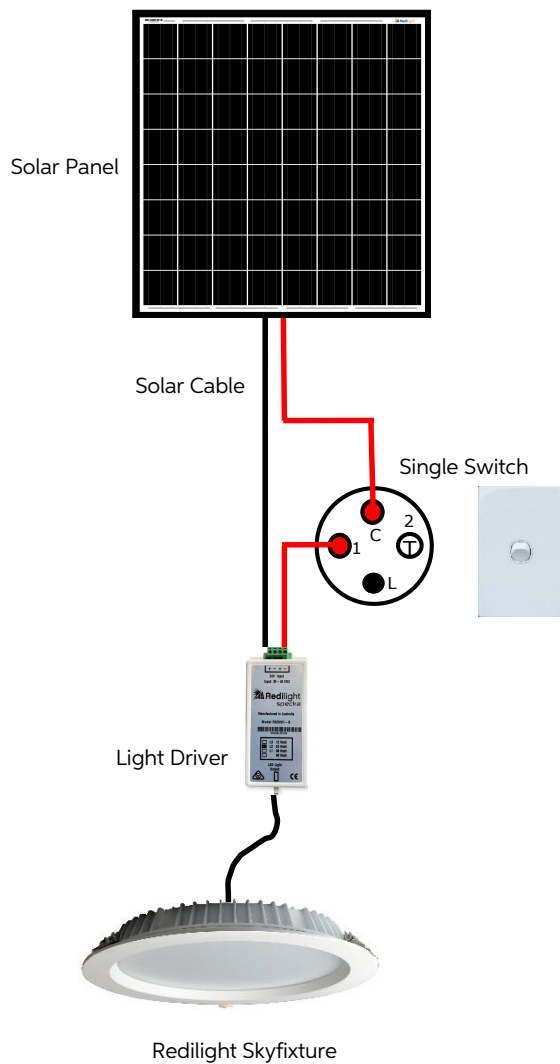
On/off switch controlling one Skyfixture
