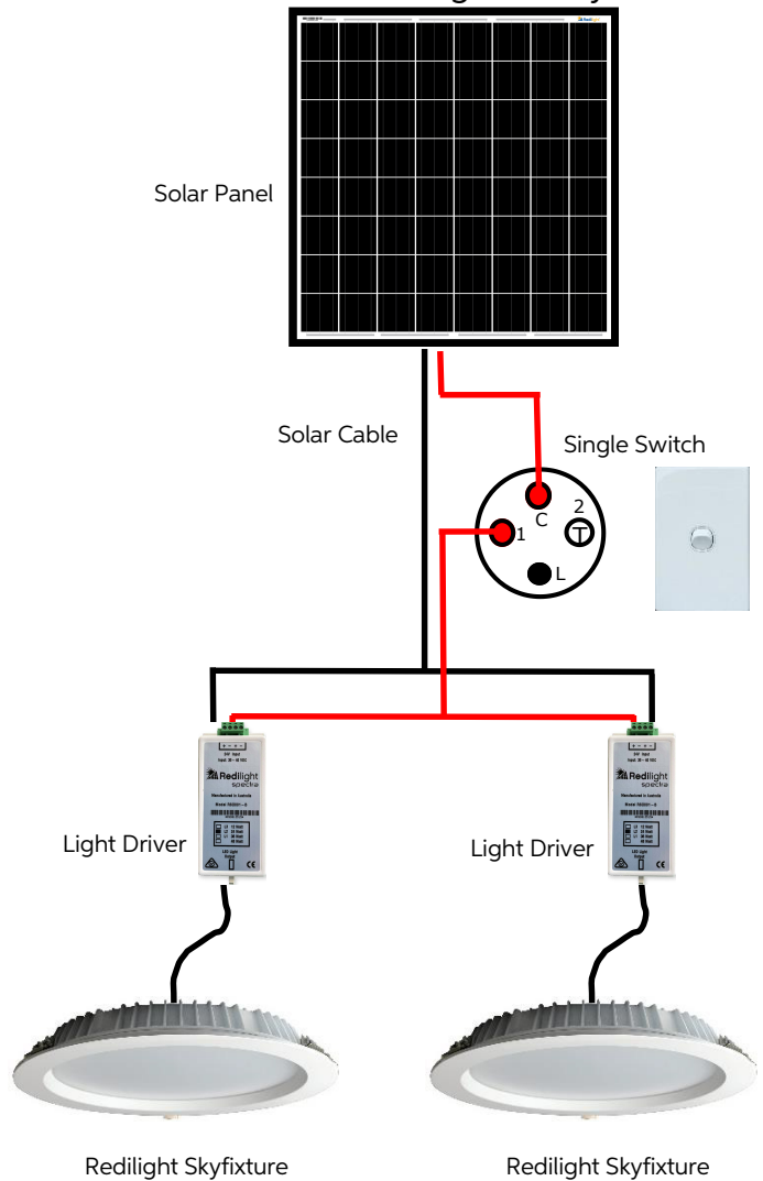
On/off switch controlling two Skyfixtures
